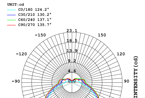
LUMINOUS INTENSITY DISTRIBUTION
