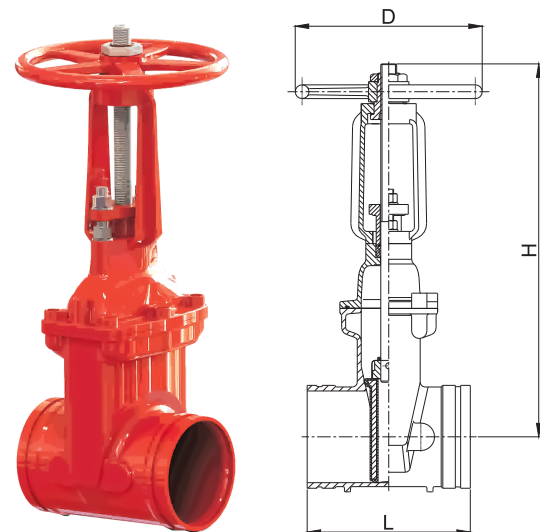
FIG. FFA-F0199-G, GR X GR Ends
