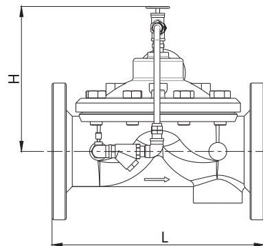
FIG. FFA-6101 FLANGED ENDS
