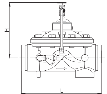
FIG. FFA-6901 GROOVED ENDS
